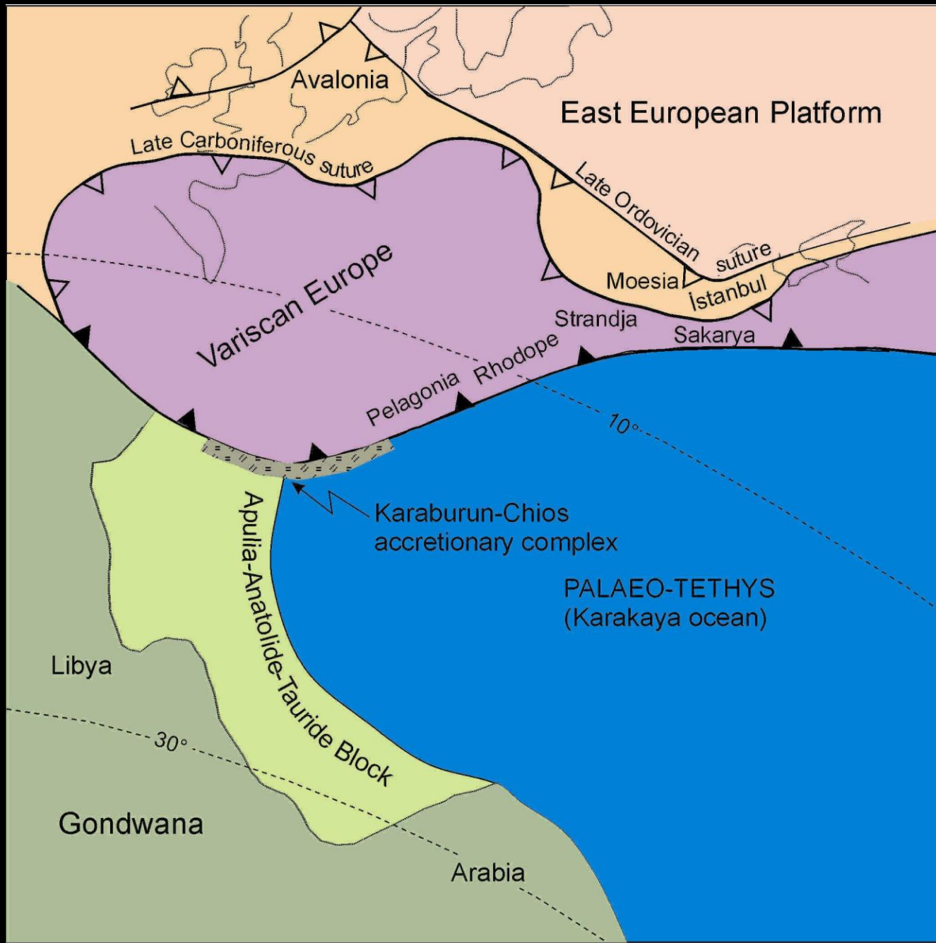
Late Carboniferous paleogeography
